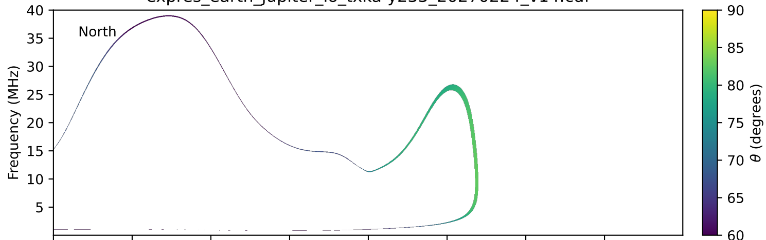
expres_earth_jupiter_io_txka-y235_20270224_v14.cdf
