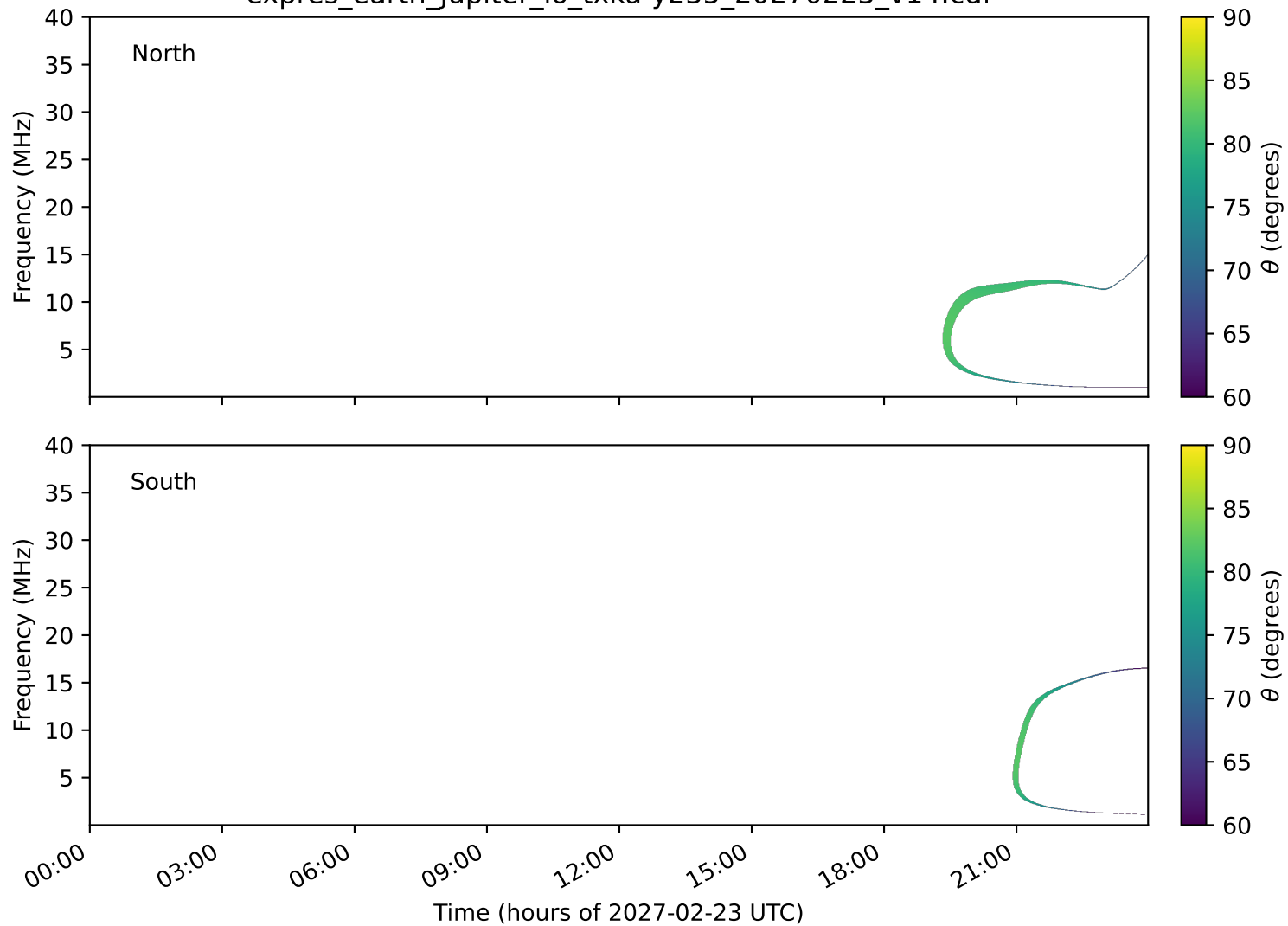
expres_earth_jupiter_io_txka-y235_20270223_v14.cdf
