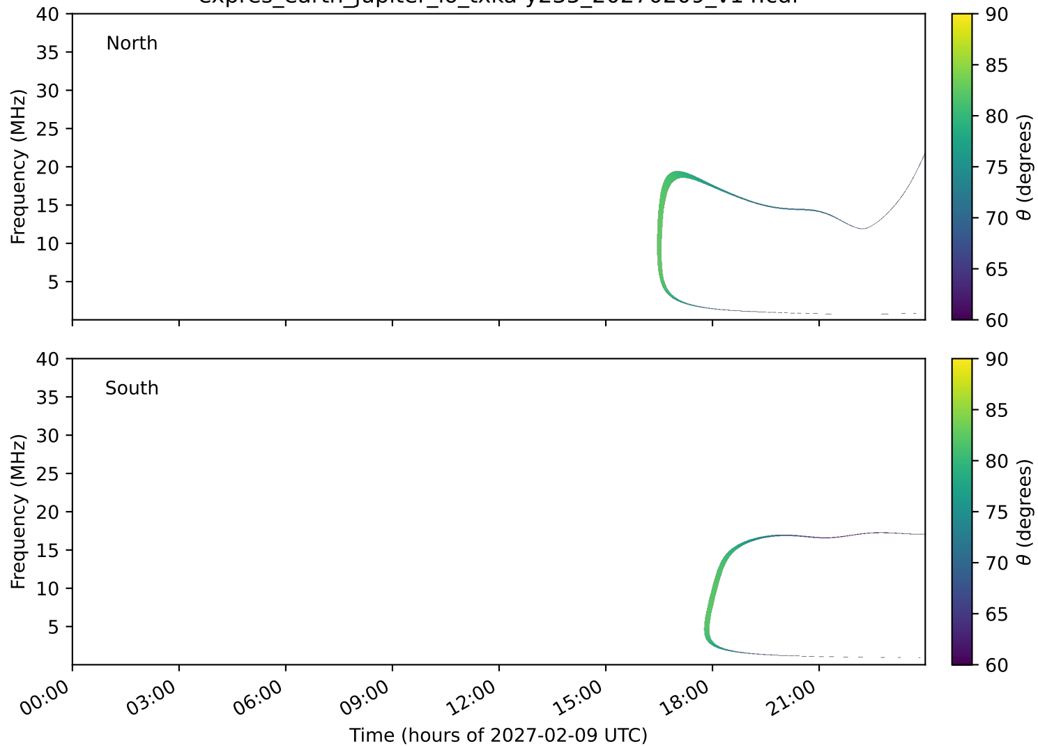
expres_earth_jupiter_io_txka-y235_20270209_v14.cdf
