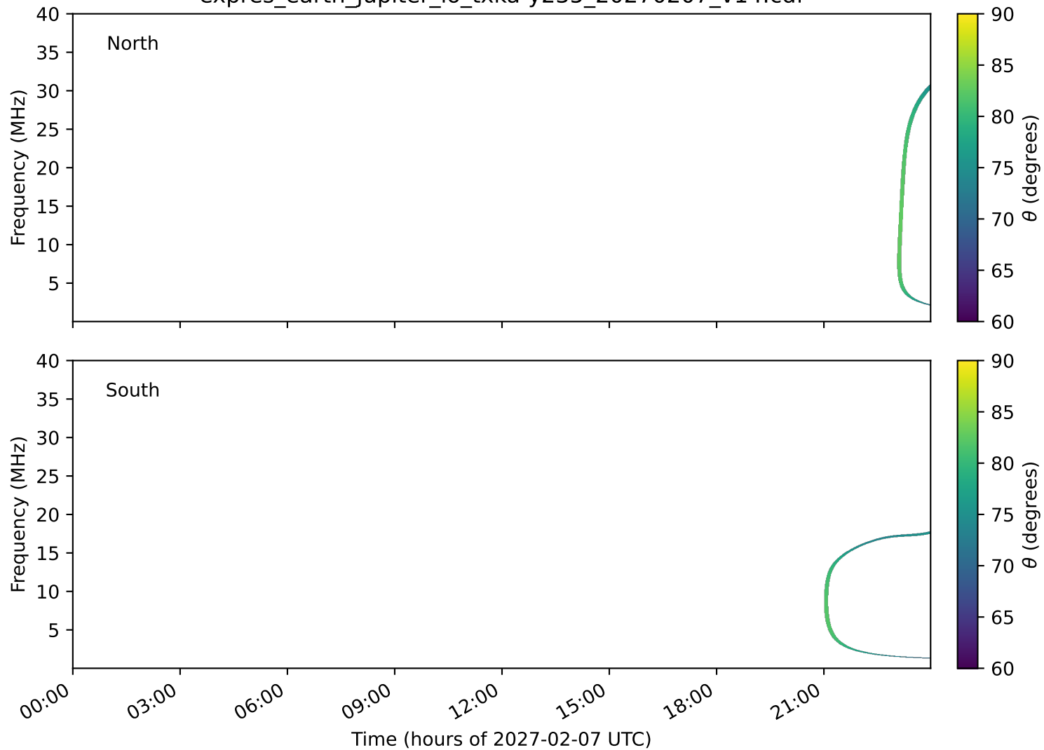
expres_earth_jupiter_io_txka-y235_20270207_v14.cdf
