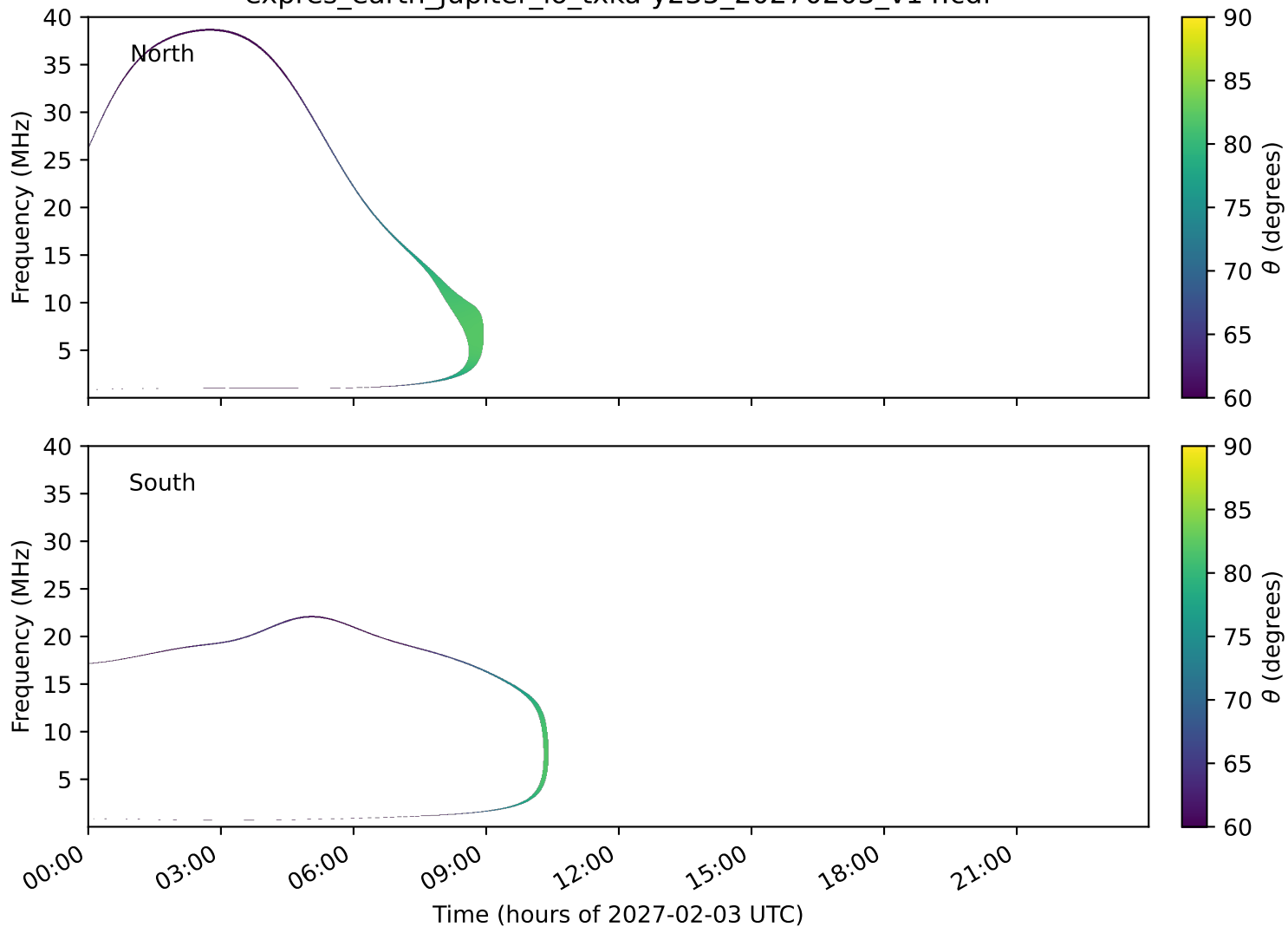
expres_earth_jupiter_io_txka-y235_20270203_v14.cdf
