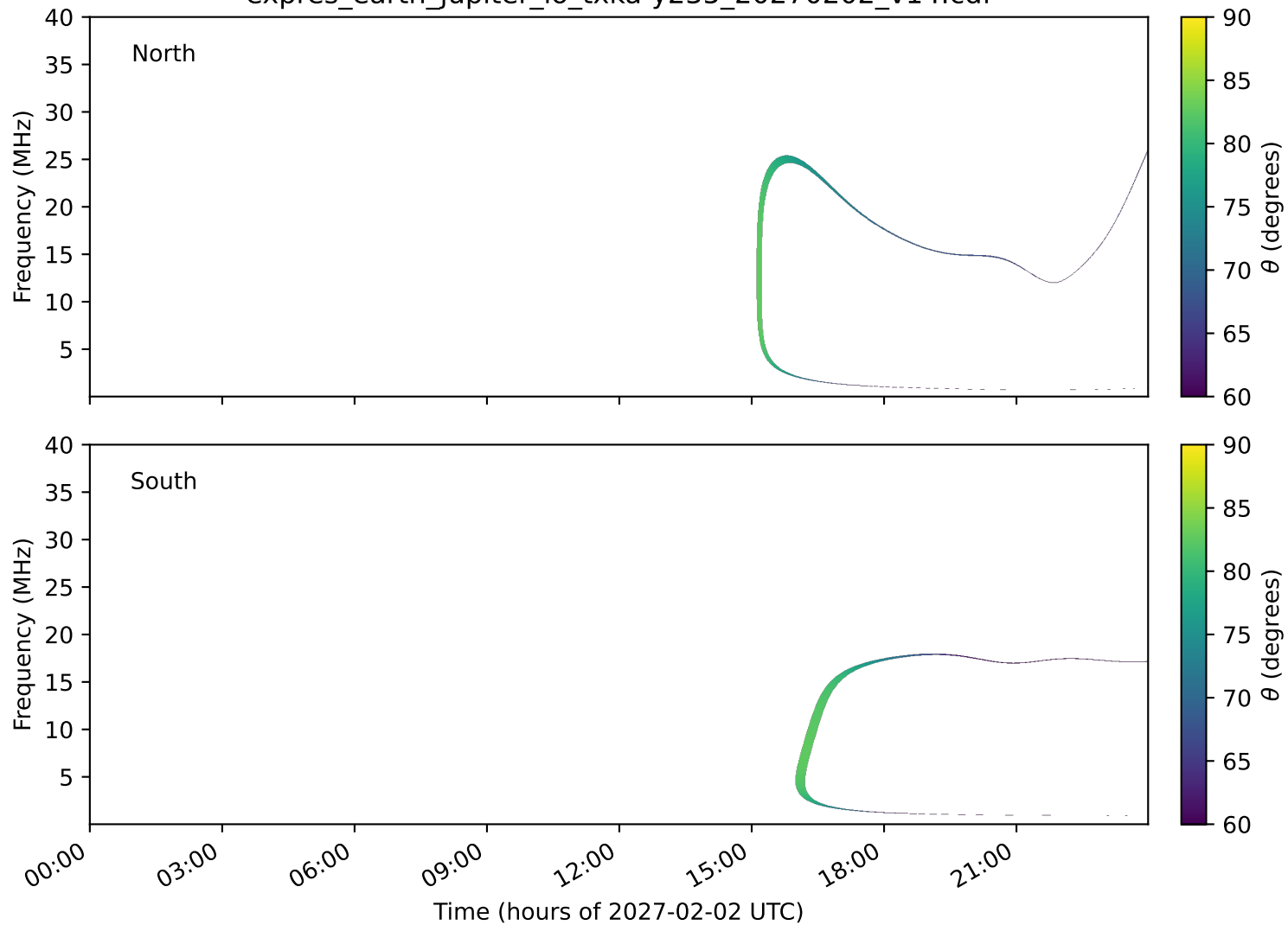
expres_earth_jupiter_io_txka-y235_20270202_v14.cdf
