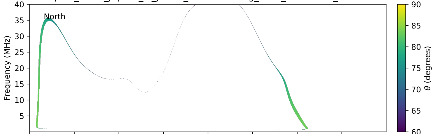
expres_earth_jupiter_io_jrm33_lossc-wid1deg_3kev_20270215_v11.cdf
