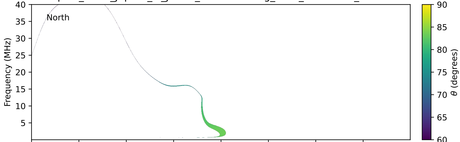
expres_earth_jupiter_io_jrm33_lossc-wid1deg_3kev_20270210_v11.cdf
