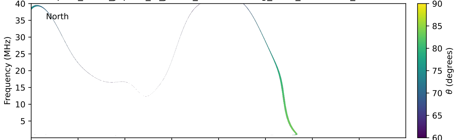
expres_earth_jupiter_io_jrm33_lossc-wid1deg_3kev_20270208_v11.cdf
