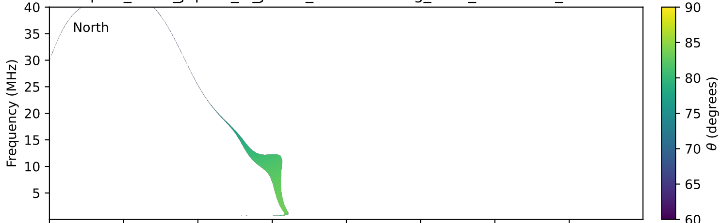
expres_earth_jupiter_io_jrm33_lossc-wid1deg_3kev_20270203_v11.cdf
