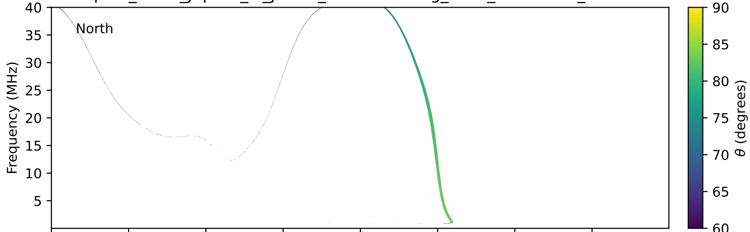
expres_earth_jupiter_io_jrm33_lossc-wid1deg_3kev_20270201_v11.cdf
