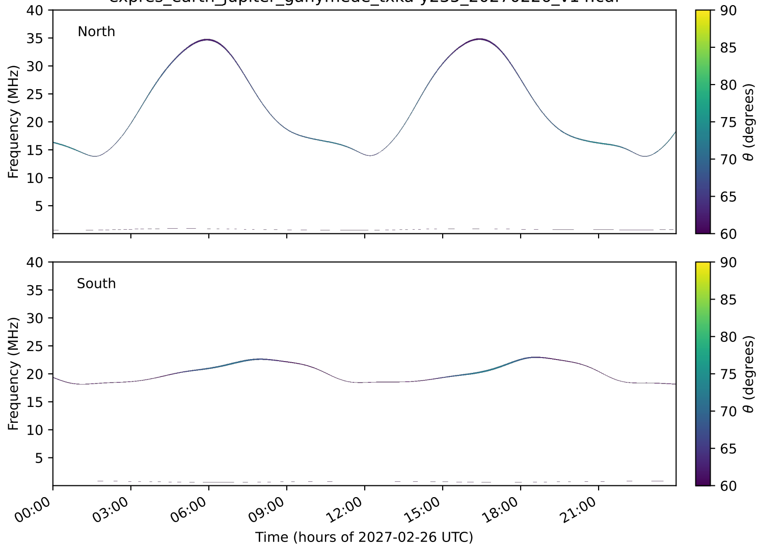
expres_earth_jupiter_ganymede_txka-y235_20270226_v14.cdf
