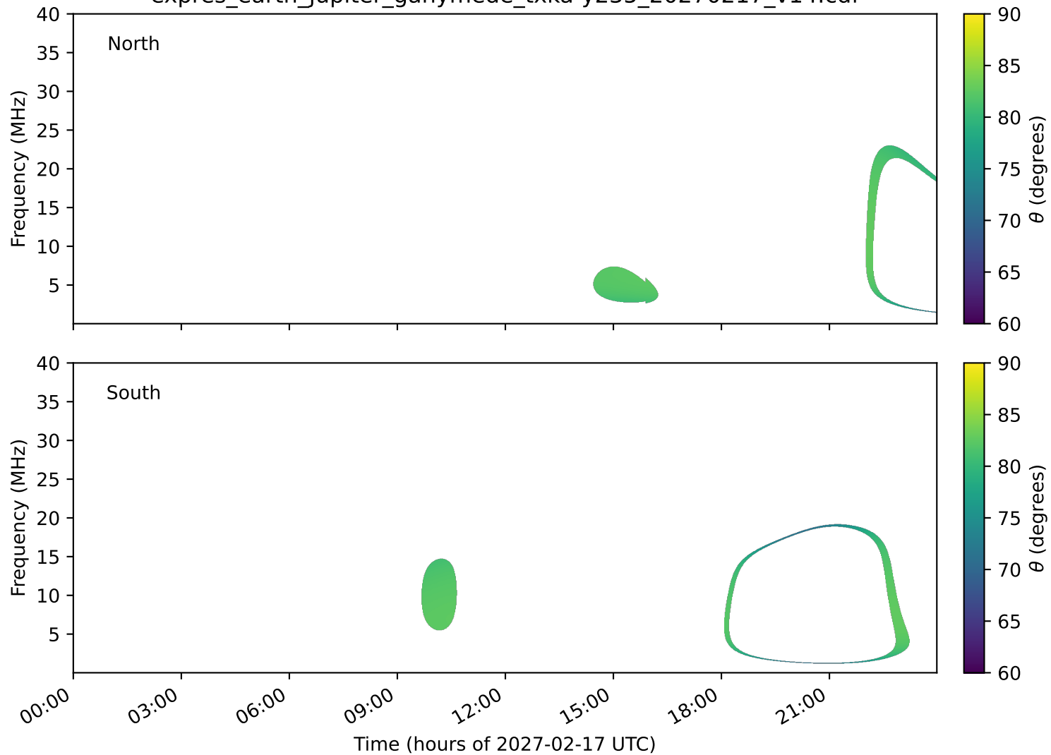
expres_earth_jupiter_ganymede_txka-y235_20270217_v14.cdf
