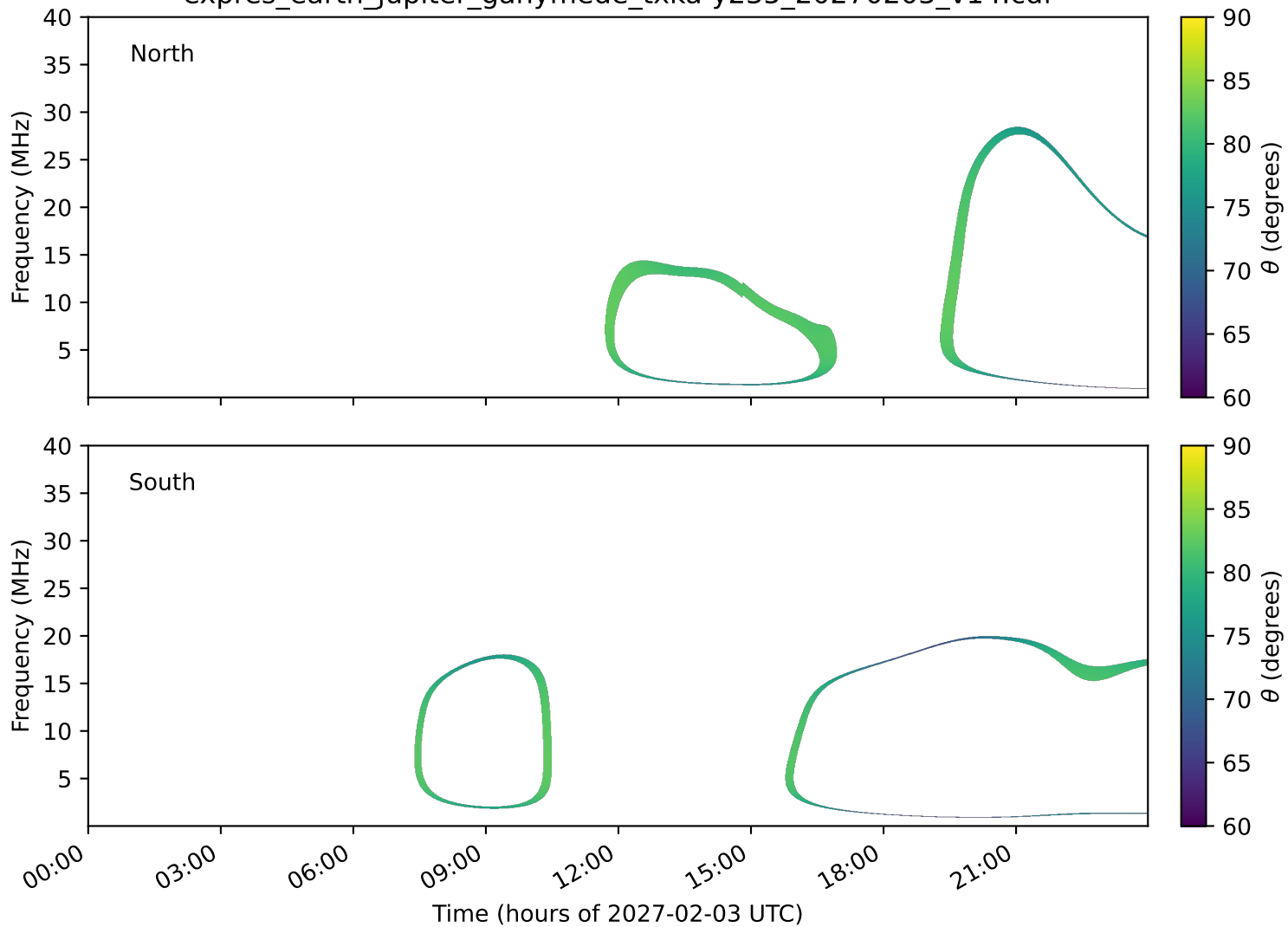
expres_earth_jupiter_ganymede_txka-y235_20270203_v14.cdf
