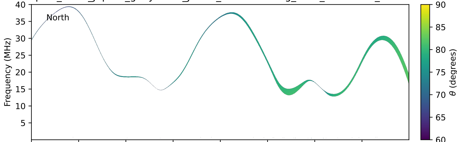
expres_earth_jupiter_ganymede_jrm33_lossc-wid1deg_3kev_20270220_v11.cdf
