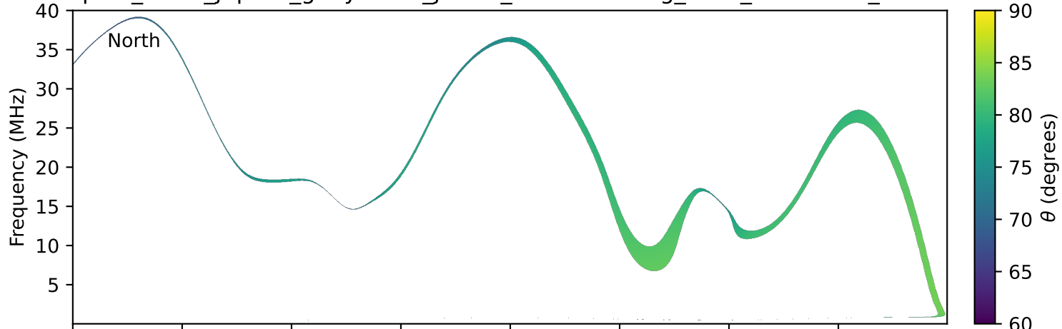
expres_earth_jupiter_ganymede_jrm33_lossc-wid1deg_3kev_20270213_v11.cdf
