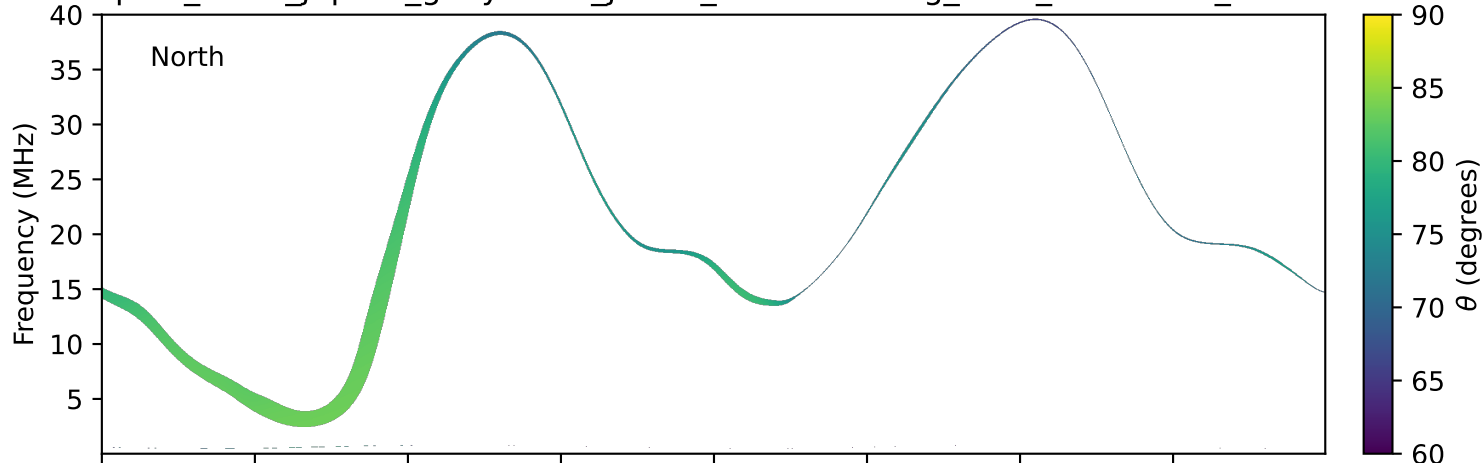
expres_earth_jupiter_ganymede_jrm33_lossc-wid1deg_3kev_20270211_v11.cdf
