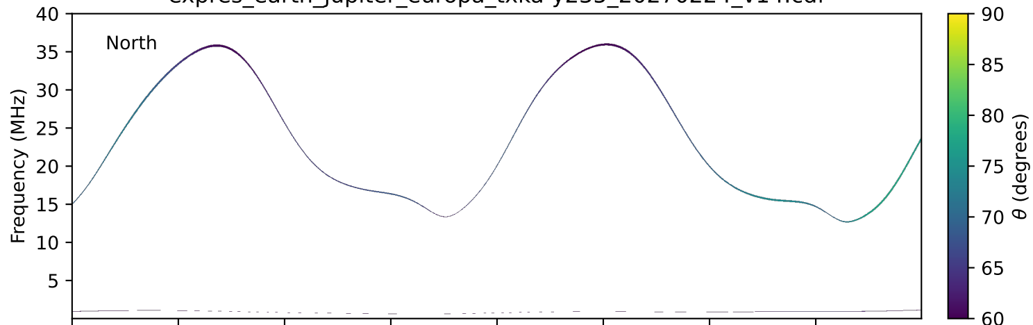
expres_earth_jupiter_europa_txka-y235_20270224_v14.cdf
