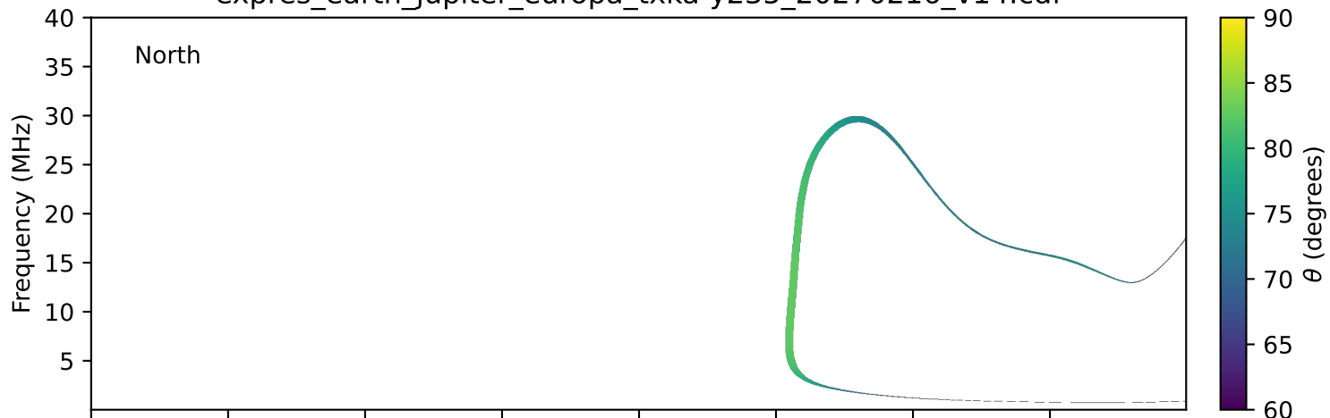
expres_earth_jupiter_europa_txka-y235_20270216_v14.cdf
