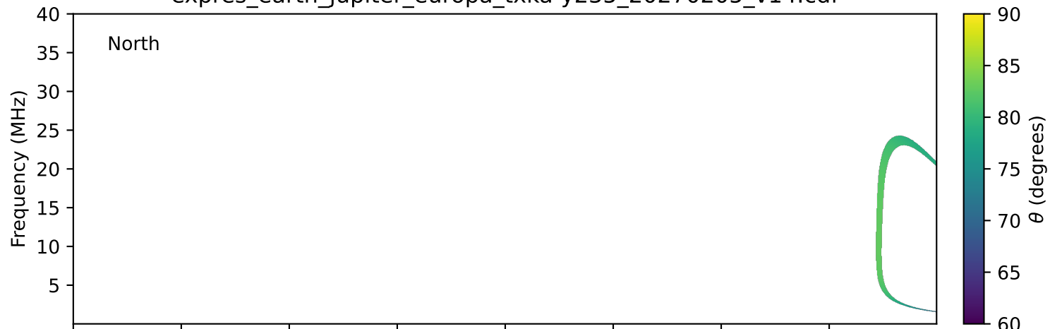
expres_earth_jupiter_europa_txka-y235_20270205_v14.cdf
