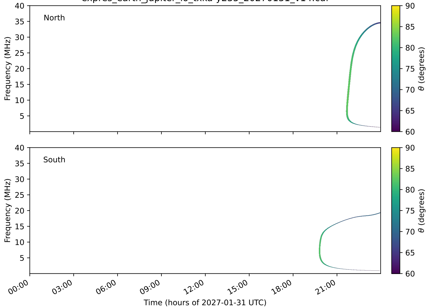
expres_earth_jupiter_io_txka-y235_20270131_v14.cdf
