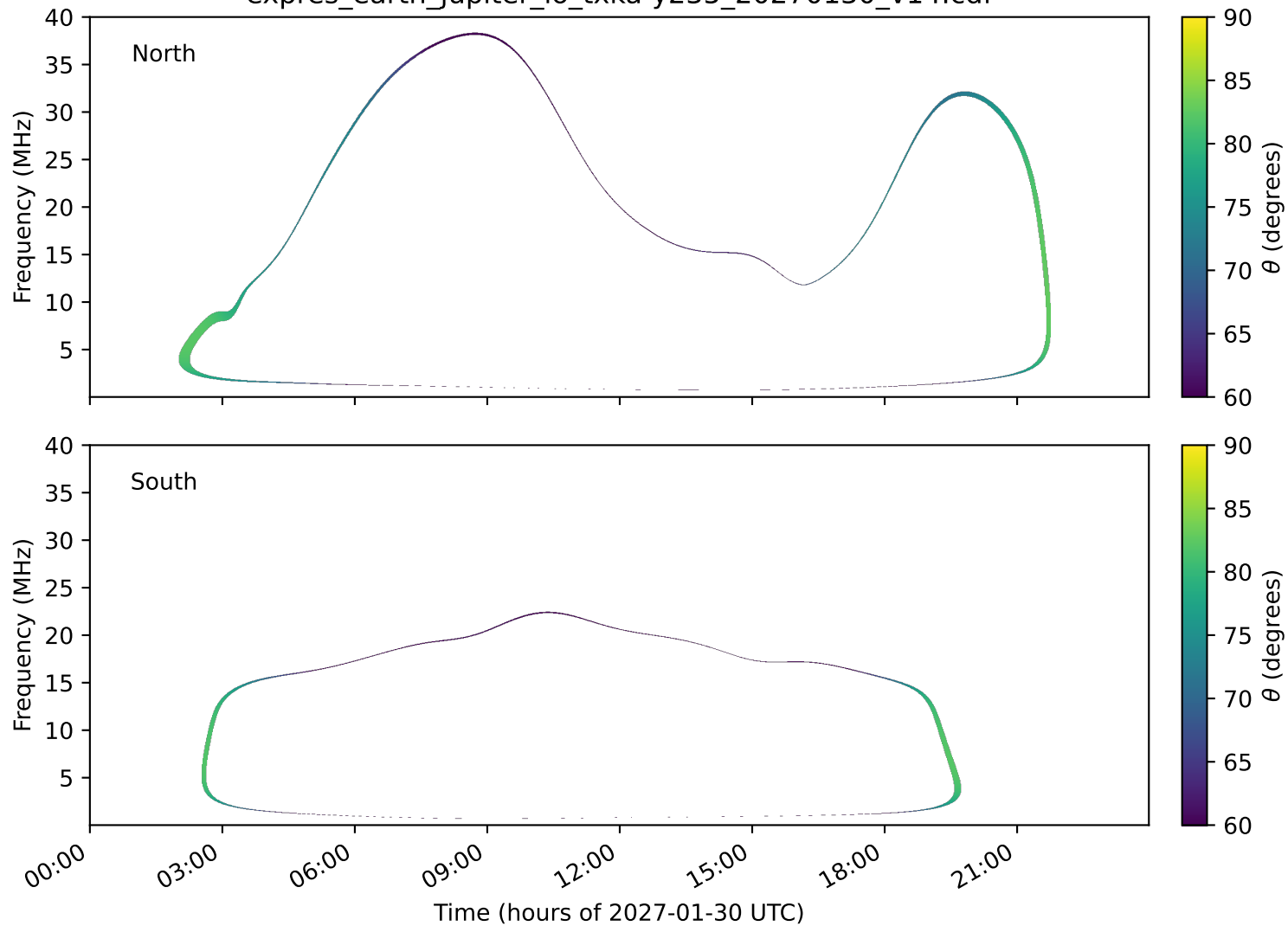
expres_earth_jupiter_io_txka-y235_20270130_v14.cdf
