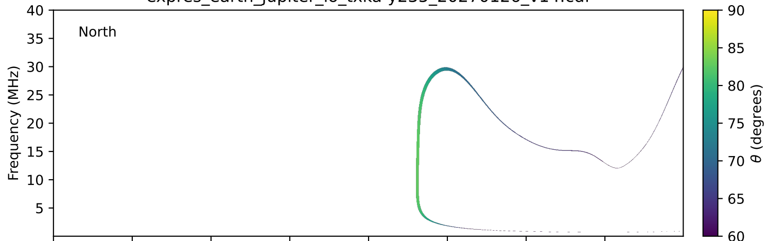
expres_earth_jupiter_io_txka-y235_20270126_v14.cdf
