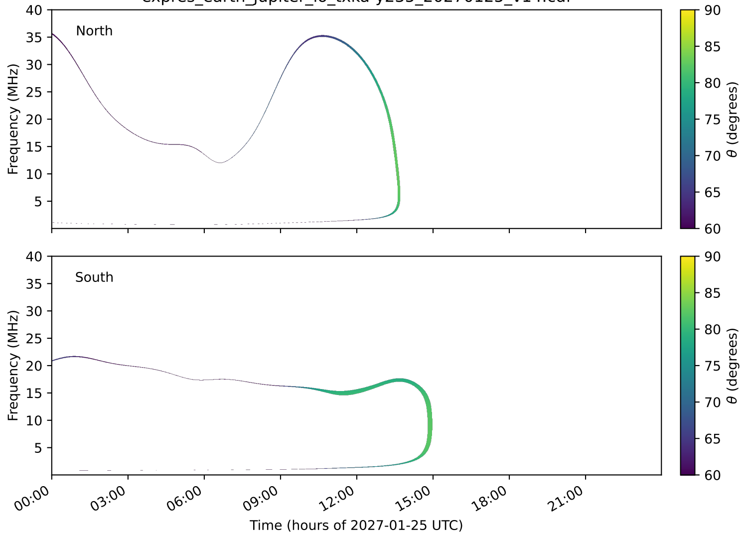
expres_earth_jupiter_io_txka-y235_20270125_v14.cdf
