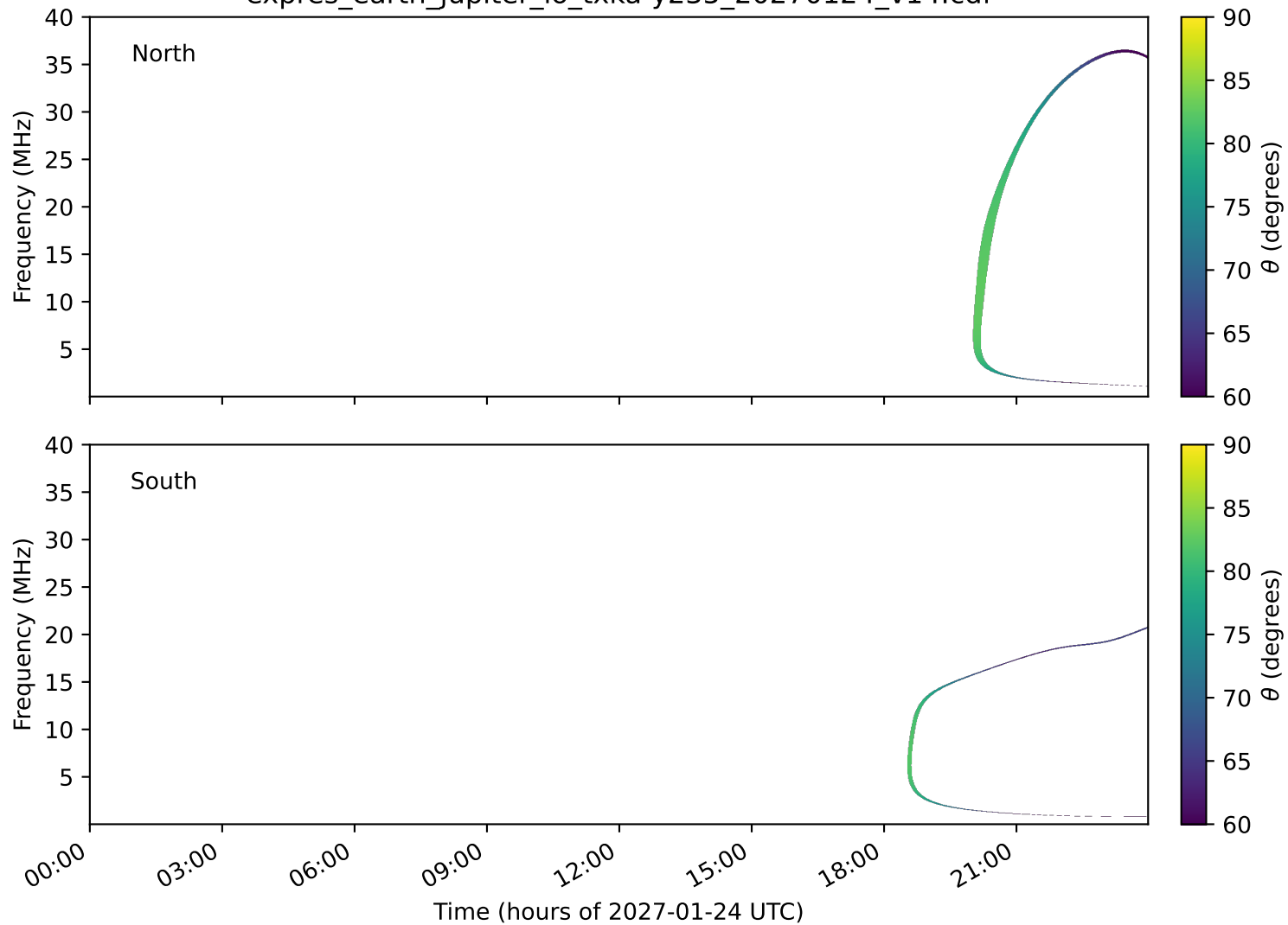
expres_earth_jupiter_io_txka-y235_20270124_v14.cdf
