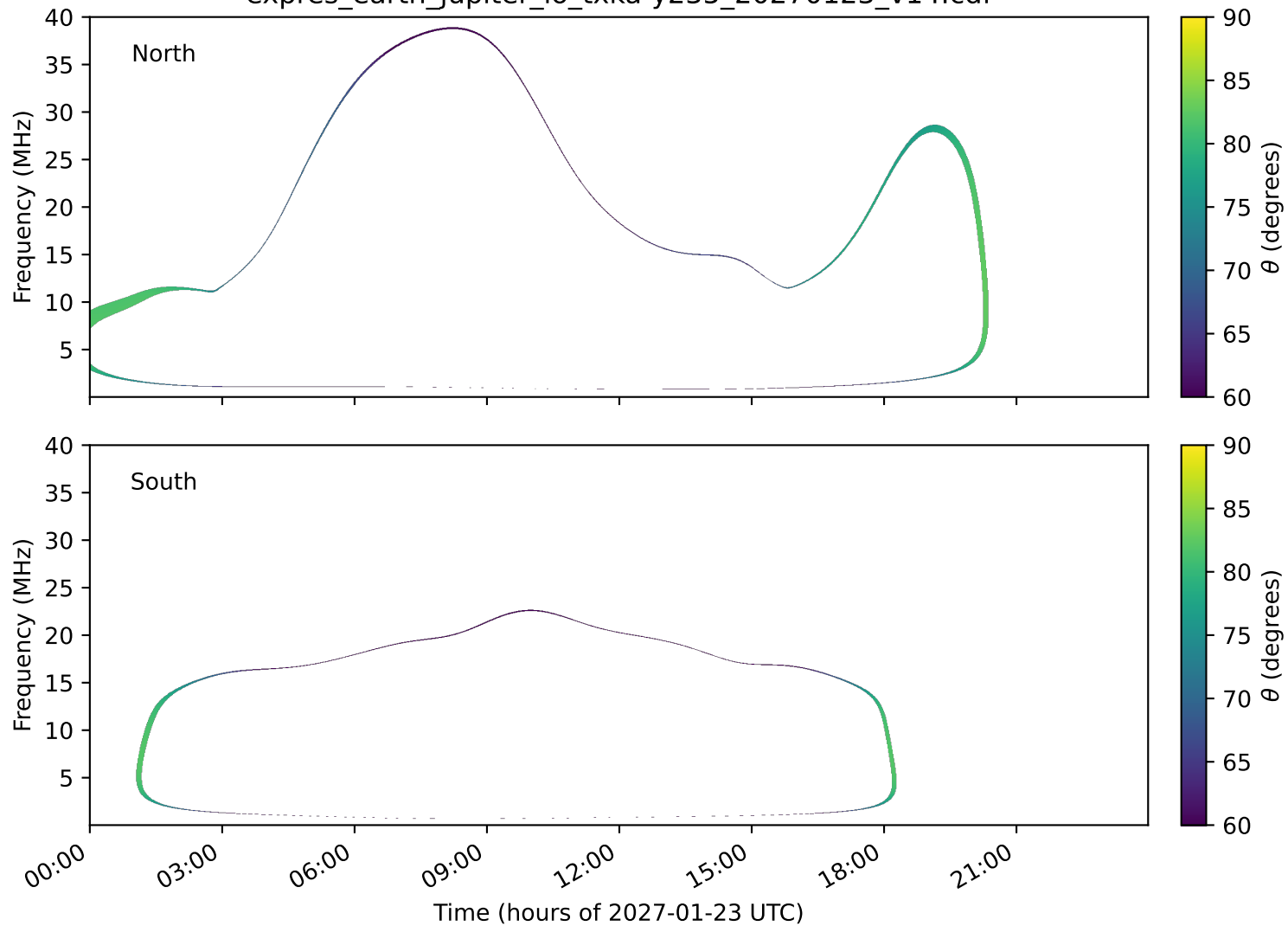
expres_earth_jupiter_io_txka-y235_20270123_v14.cdf
