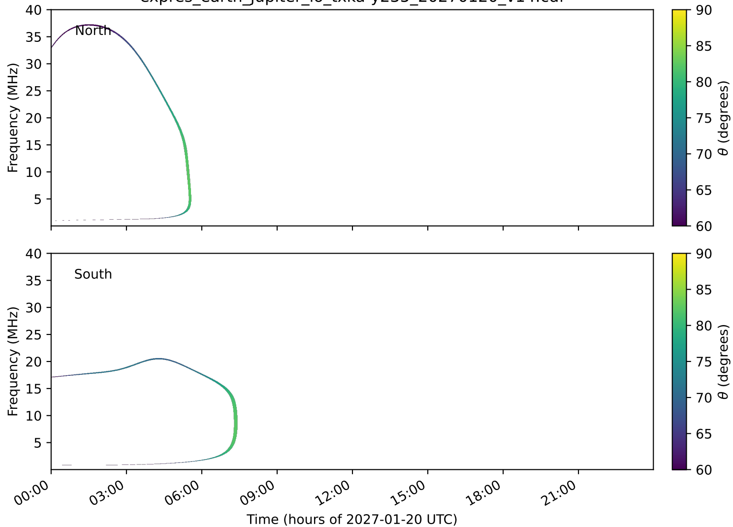
expres_earth_jupiter_io_txka-y235_20270120_v14.cdf
