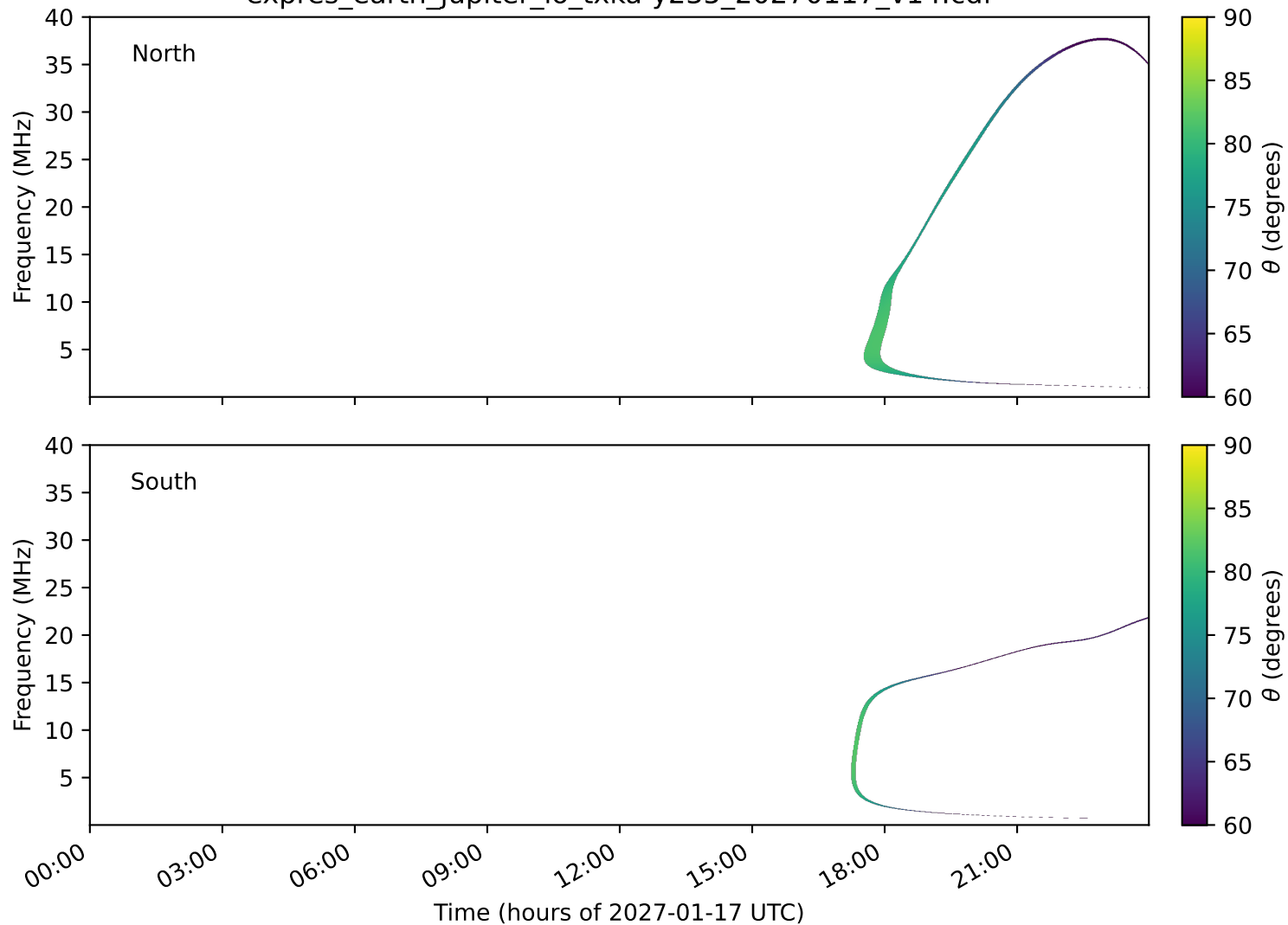
expres_earth_jupiter_io_txka-y235_20270117_v14.cdf
