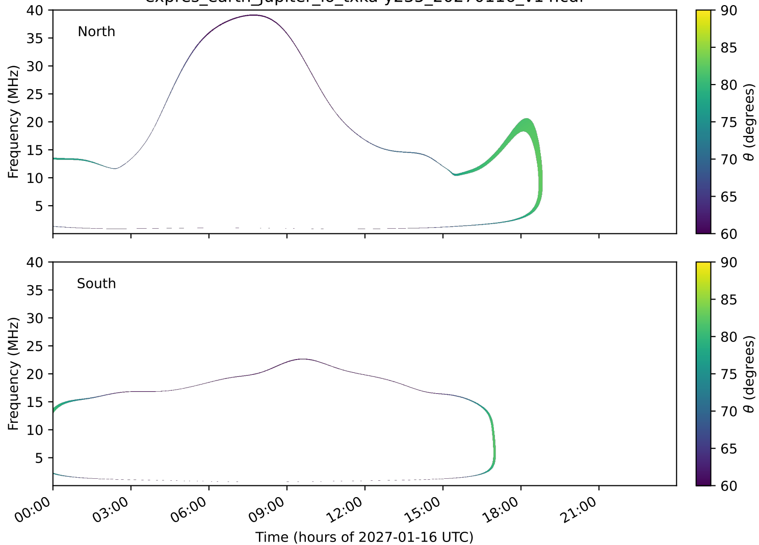
expres_earth_jupiter_io_txka-y235_20270116_v14.cdf
