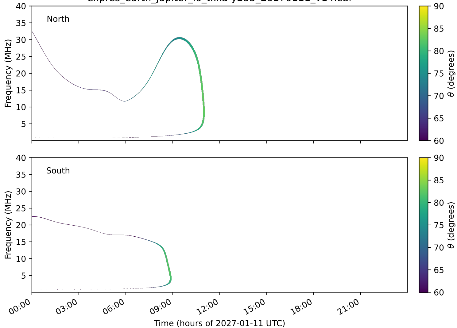
expres_earth_jupiter_io_txka-y235_20270111_v14.cdf
