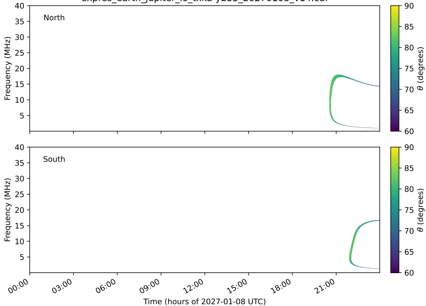
expres_earth_jupiter_io_txka-y235_20270108_v14.cdf
