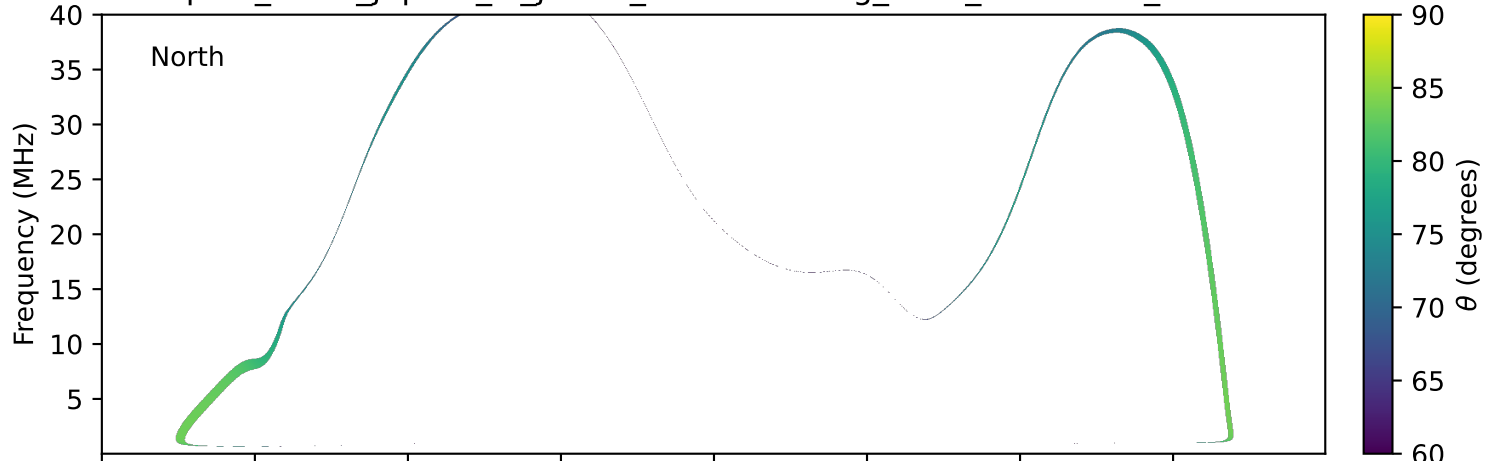
expres_earth_jupiter_io_jrm33_lossc-wid1deg_3kev_20270130_v11.cdf
