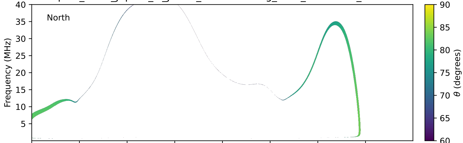
expres_earth_jupiter_io_jrm33_lossc-wid1deg_3kev_20270123_v11.cdf
