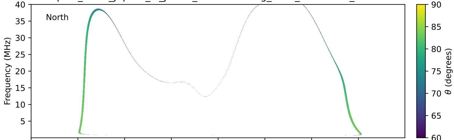
expres_earth_jupiter_io_jrm33_lossc-wid1deg_3kev_20270107_v11.cdf
