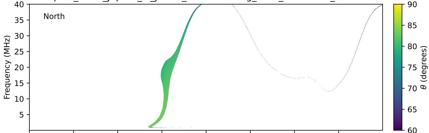
expres_earth_jupiter_io_jrm33_lossc-wid1deg_3kev_20270105_v11.cdf
