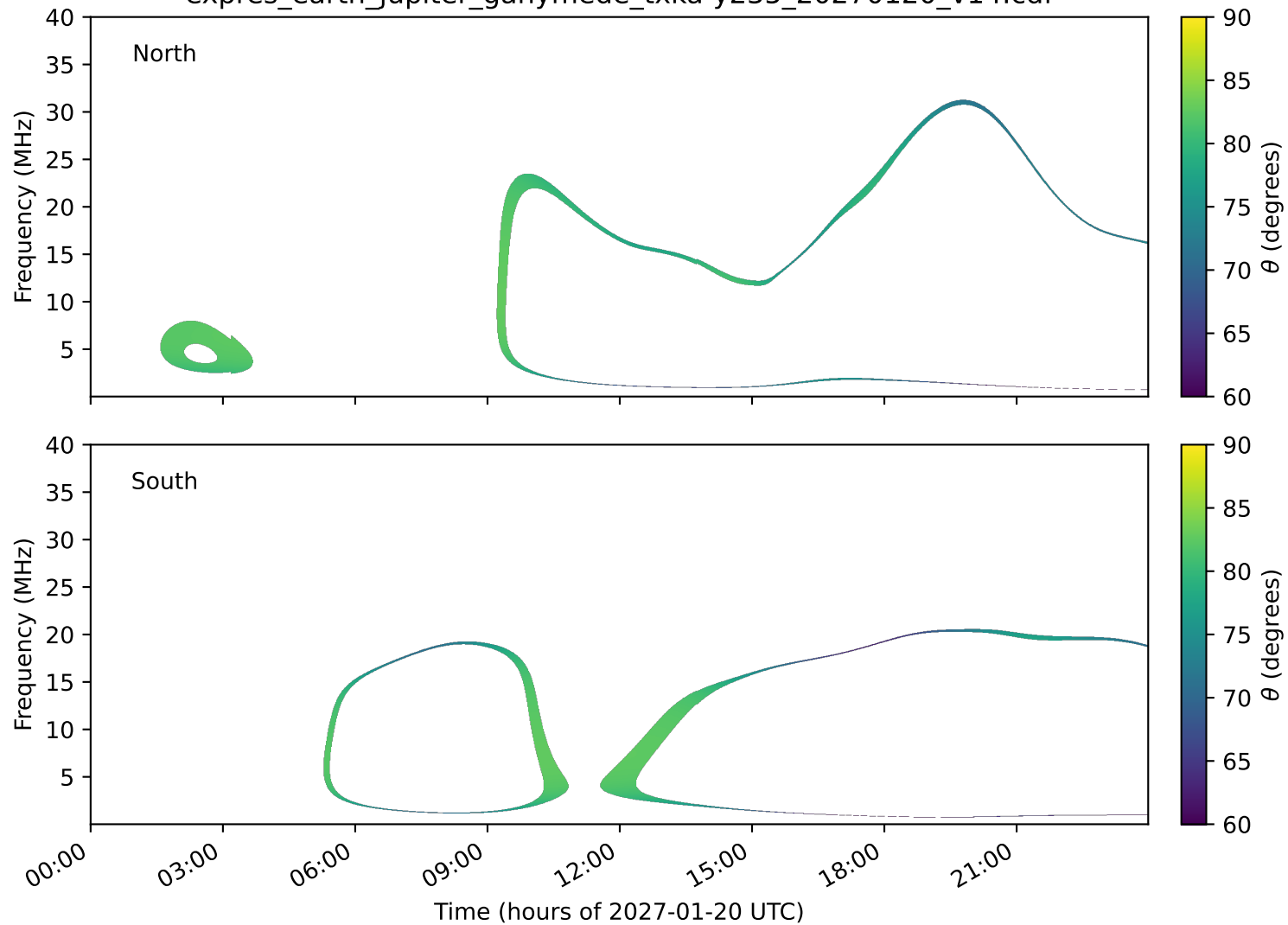
expres_earth_jupiter_ganymede_txka-y235_20270120_v14.cdf
