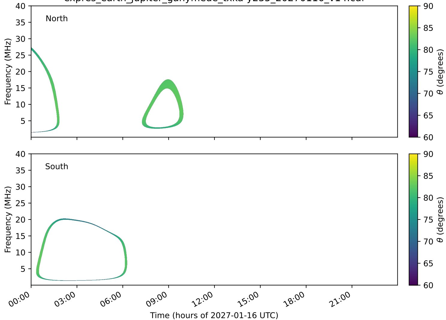
expres_earth_jupiter_ganymede_txka-y235_20270116_v14.cdf
