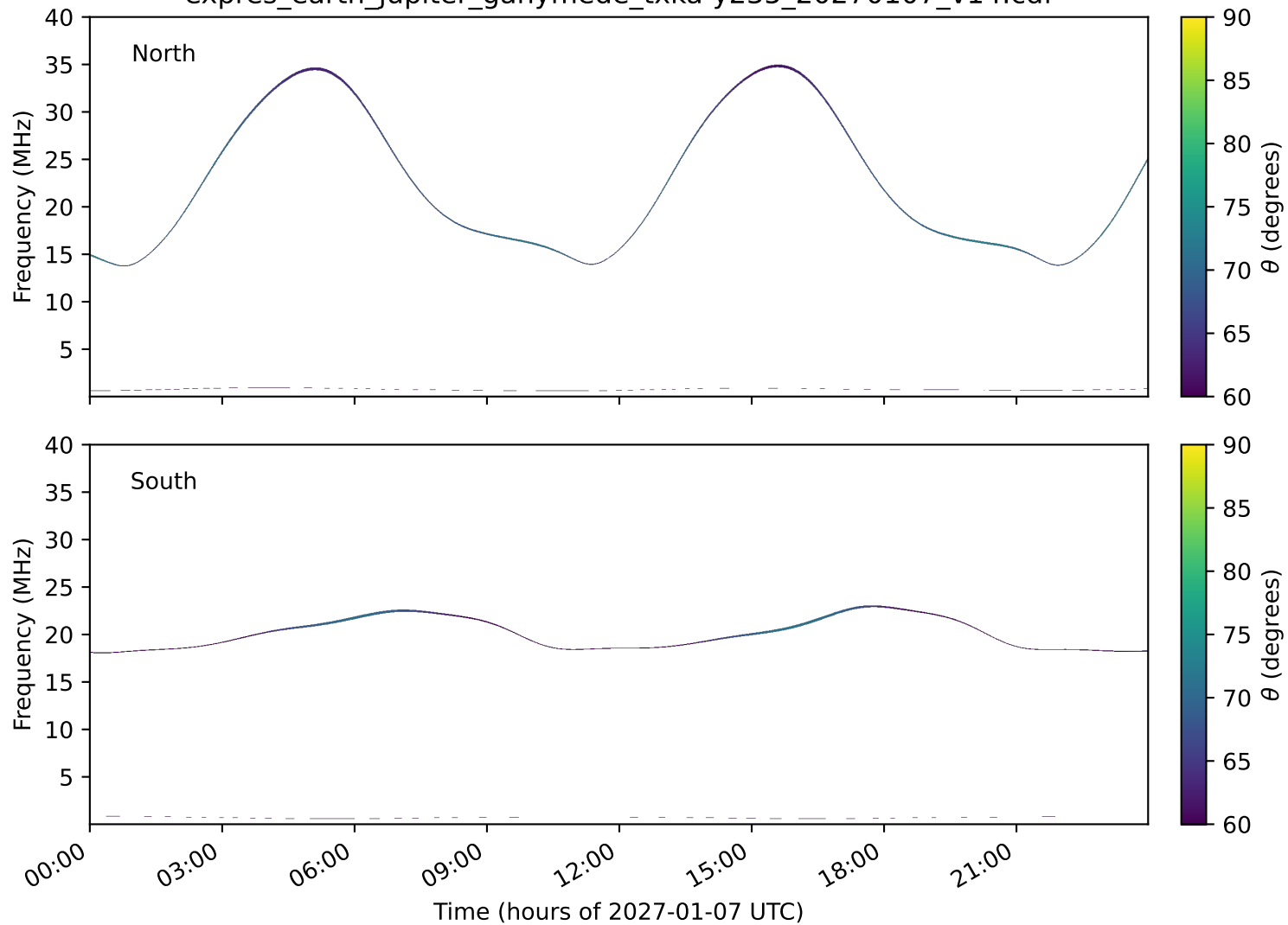
expres_earth_jupiter_ganymede_txka-y235_20270107_v14.cdf
