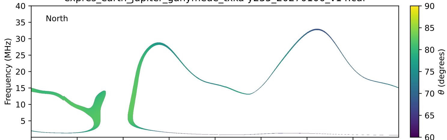
expres_earth_jupiter_ganymede_txka-y235_20270106_v14.cdf
