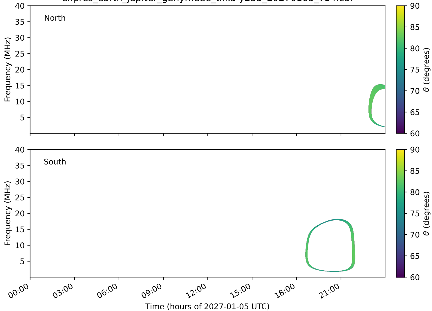
expres_earth_jupiter_ganymede_txka-y235_20270105_v14.cdf
