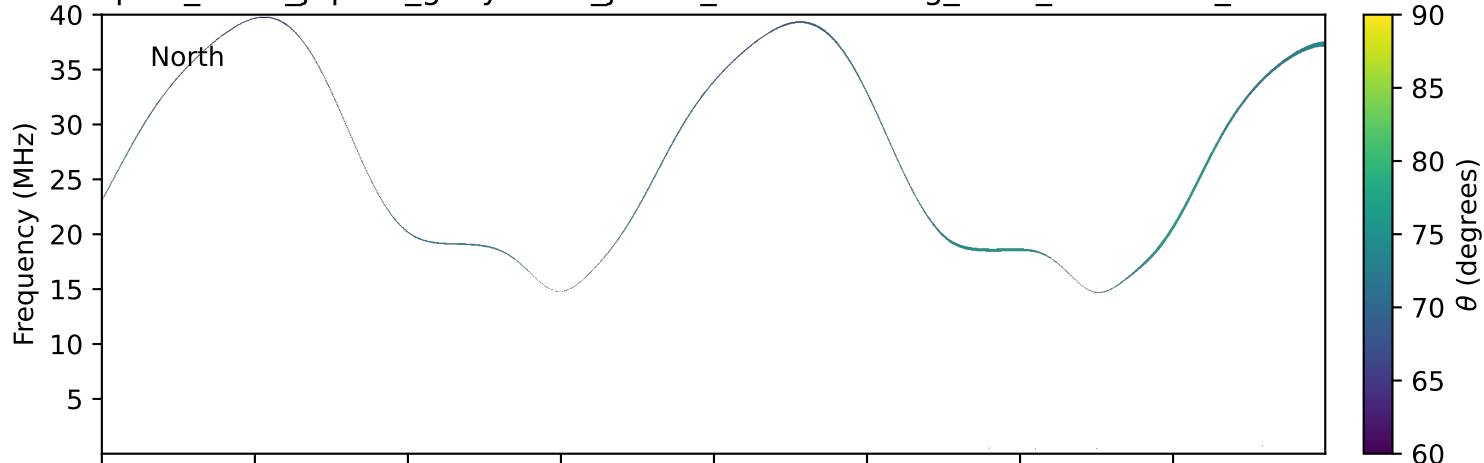
expres_earth_jupiter_ganymede_jrm33_lossc-wid1deg_3kev_20270122_v11.cdf
