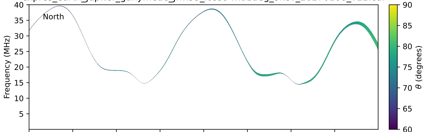
expres_earth_jupiter_ganymede_jrm33_lossc-wid1deg_3kev_20270108_v11.cdf
