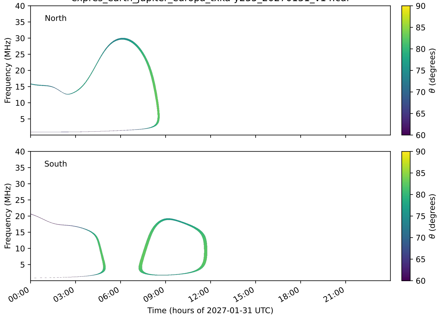
expres_earth_jupiter_europa_txka-y235_20270131_v14.cdf
