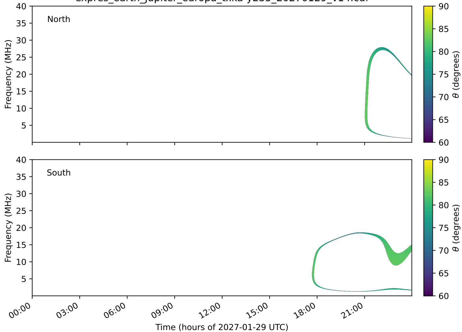
expres_earth_jupiter_europa_txka-y235_20270129_v14.cdf
