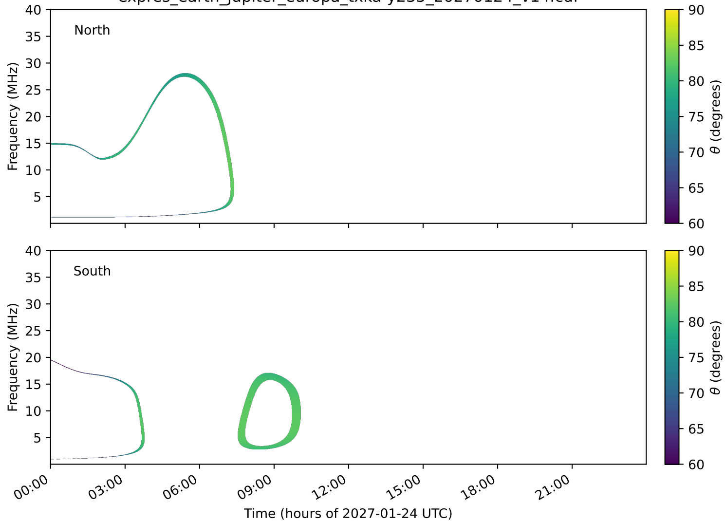
expres_earth_jupiter_europa_txka-y235_20270124_v14.cdf
