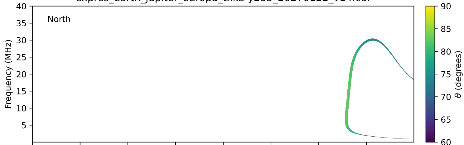
expres_earth_jupiter_europa_txka-y235_20270122_v14.cdf
