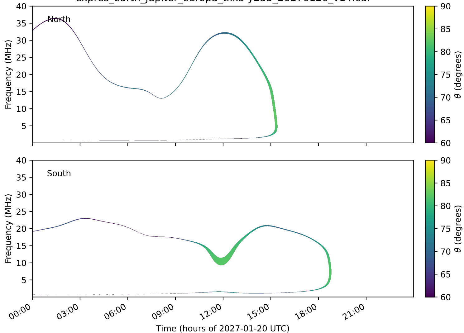
expres_earth_jupiter_europa_txka-y235_20270120_v14.cdf
