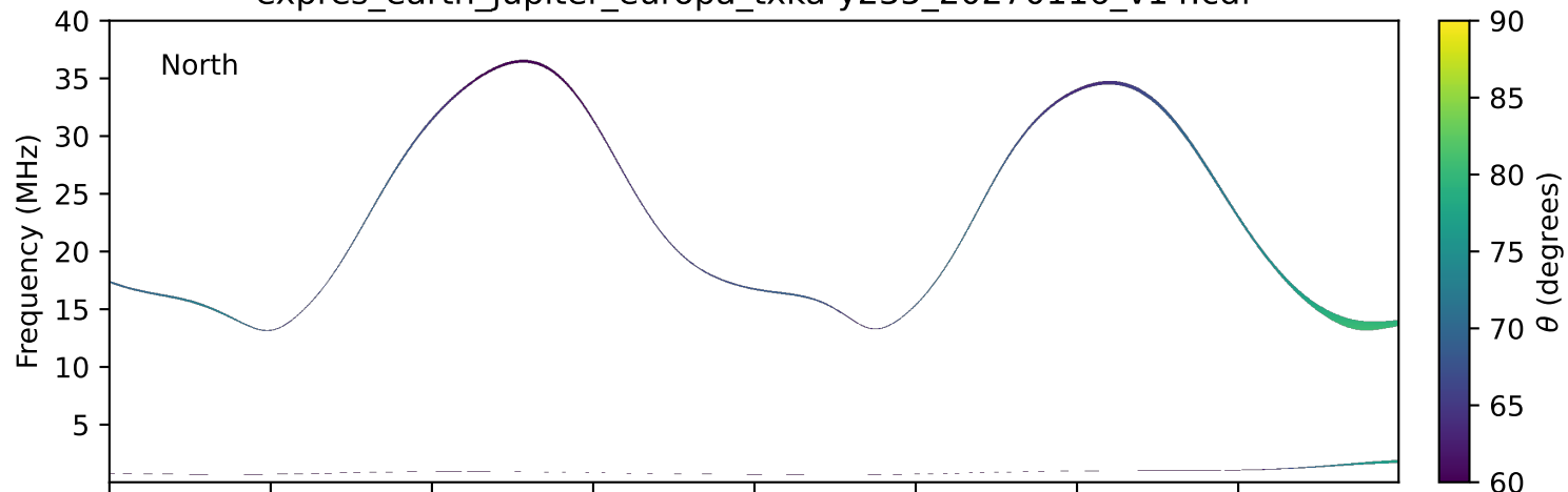
expres_earth_jupiter_europa_txka-y235_20270116_v14.cdf
