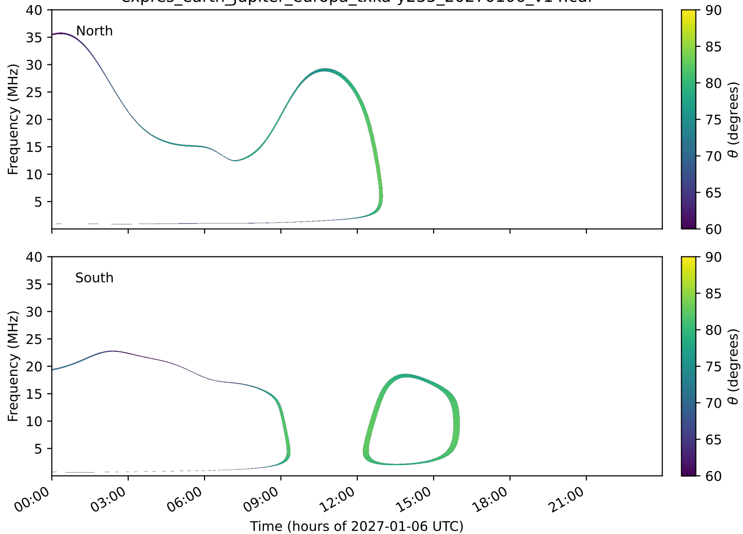
expres_earth_jupiter_europa_txka-y235_20270106_v14.cdf
