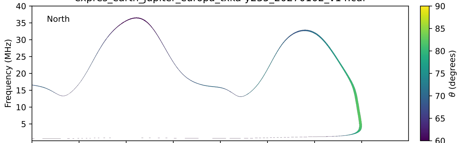
expres_earth_jupiter_europa_txka-y235_20270102_v14.cdf
